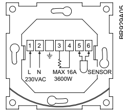
Connections
