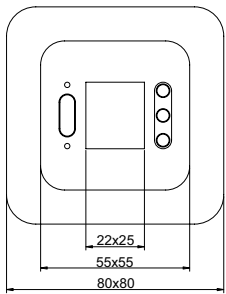
Dimensions (mm)
